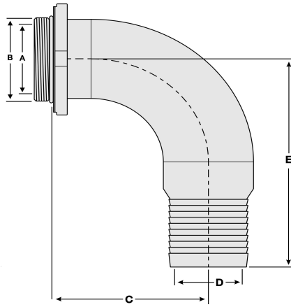
O-RING SEALED ADAPTER TO LONG RADIUS 90 DEGREES ELBOW TO HOSE BARB
