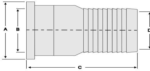
O-RING SEALED ADAPTER TO HOSE BARB
